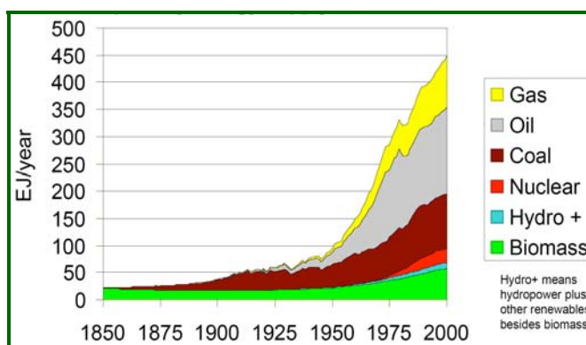
Figure 3.1: Worldwide Use of Energy from 1850 to 2000 1
